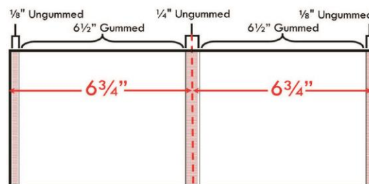
Pattern for Tire Label TLL2511E4Q Slit Sizes 6 3/4", 13 1/2"
